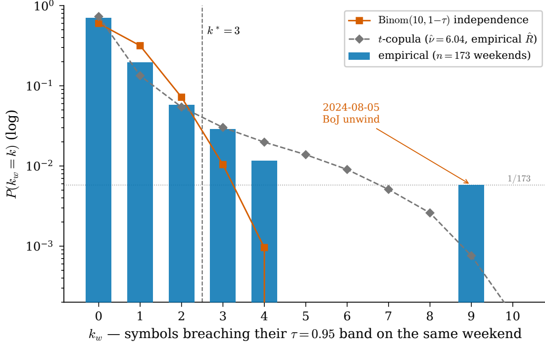
Figure 5: The joint-tail distribution at \tau = 0.95 : empirical P(k_w = k) over the 173 OOS weekends (blue bars) against the Binom( 10, 1-\tau ) independence strawman (vermilion) and the fitted Student- t copula ( \hat{\nu} = 6.04 , empirical \hat{R} ; grey dashed), log scale. The empirical mass at k \geq 3 sits a factor \sim 3 – 10\times above independence — the variance overdispersion in one picture — while remaining inside the t-copula envelope from below. The reserve-guidance threshold k^* = 3 and the single k_w = 9 weekend (2024-08-05 BoJ unwind; Fig. 6) are marked; under independence that weekend is a \sim 10^{-4} event, under the t-copula \sim 10^{-3} . No incumbent oracle publishes this distribution.
